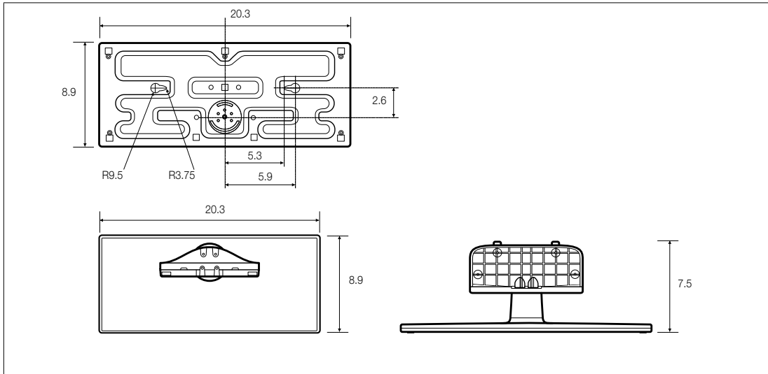
HG40NA577 / HG46NA577 Base Stand detail
